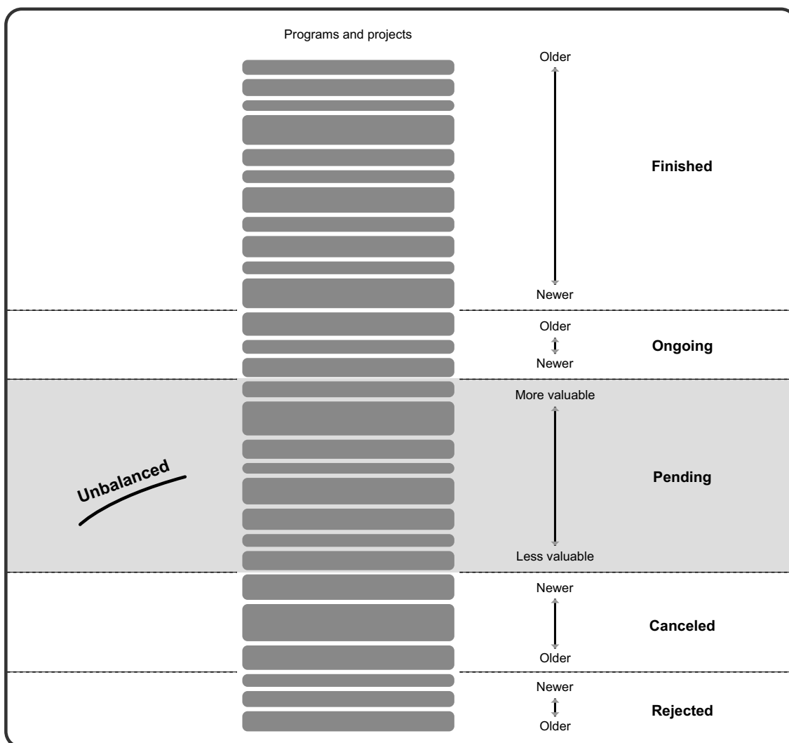
The initial ordering of the Value Generation Matrix
